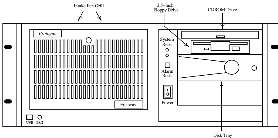
Figure 3-1. Front View, Freeway 3410 (half-width door not shown)
