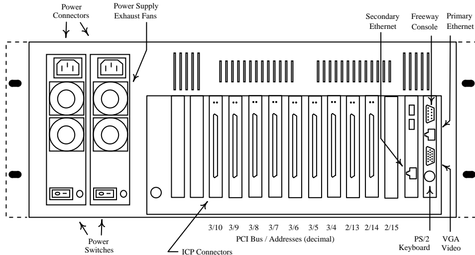
Figure 3-2. Rear View, Freeway 3410 (Redundant Power Supply Configuration)
