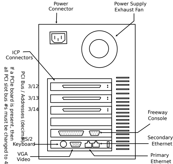
Figure 3-2. Rear View, Freeway 215
