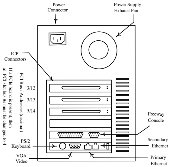
Figure 3-2. Rear View, Freeway 214
