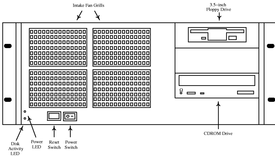
Figure 3-1. Front View, Freeway 3400 (full-width door not shown)
