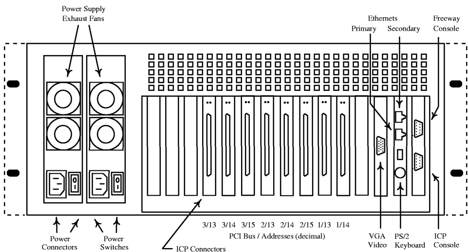
Figure 3-2. Rear View, Freeway 3400 (Redundant Power Supply Configuration)
