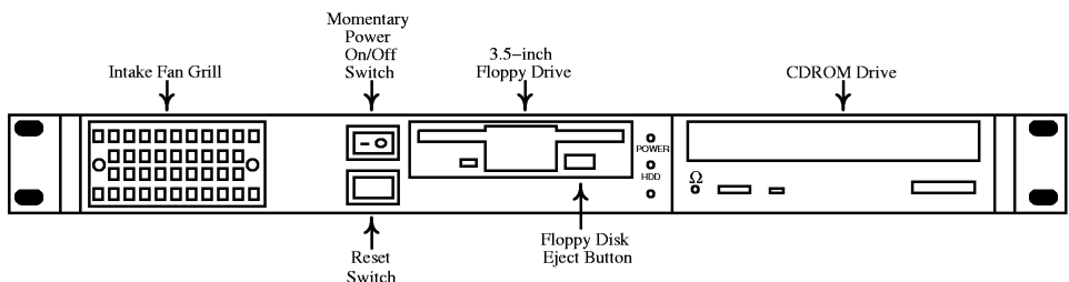
Figure 3-1. Front View, Freeway 500 (full-width door not shown)
