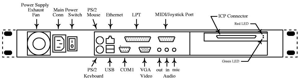
Figure 3-2. Rear View, Freeway 500
