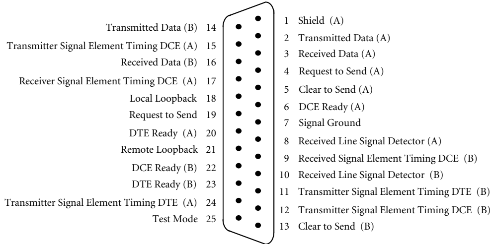
Figure 2: Signal Mapping for the 25-pin EIA-530 Interface
