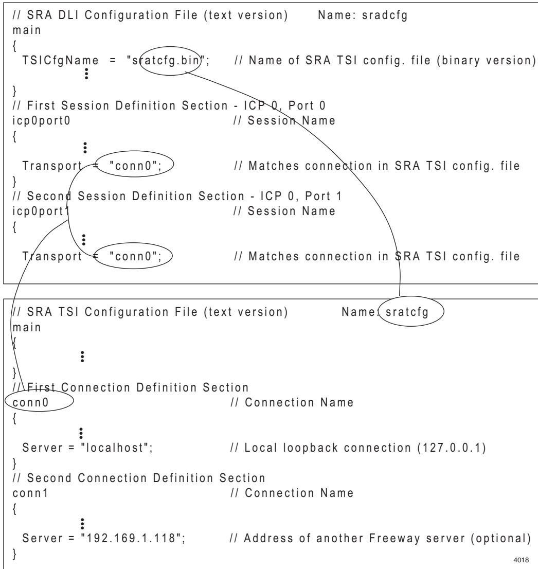
Figure 3–2: Connection between DLI and TSI configuration files
