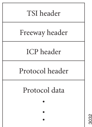
Figure 6–2: Freeway Server Message Buffer
