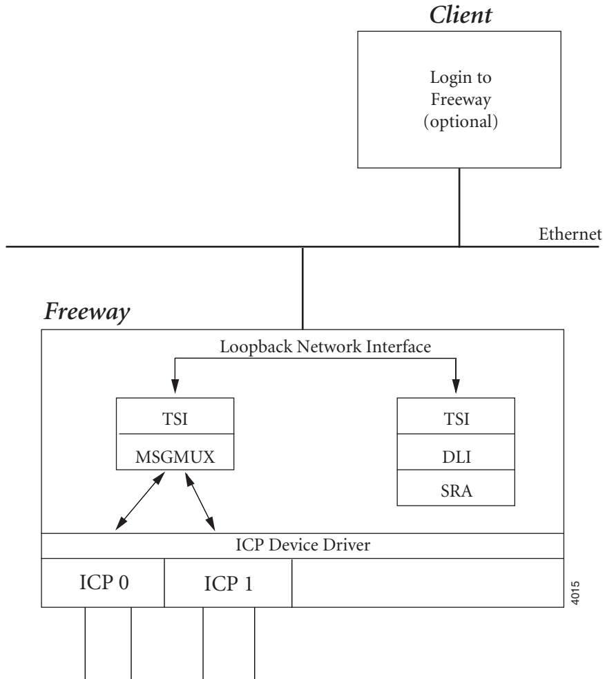
Figure 1-3: Example of an SRA Protocol Converter
