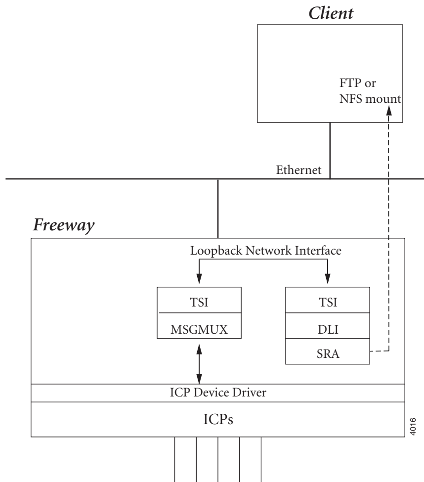
Figure 1-4: Example of a NON-API Client Interface
