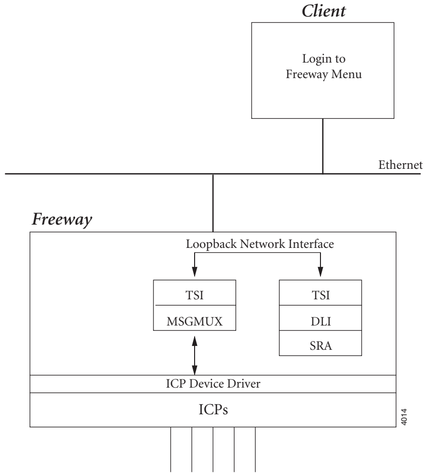
Figure 1-2: Example of a Basic SRA
